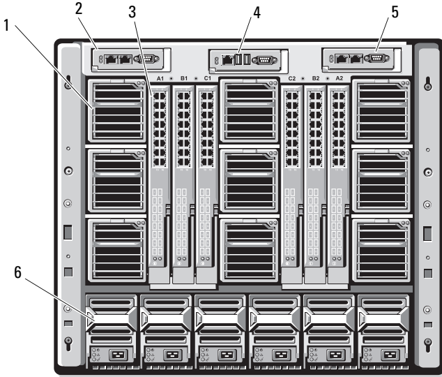
Figure 1-6. Back-Panel Features
